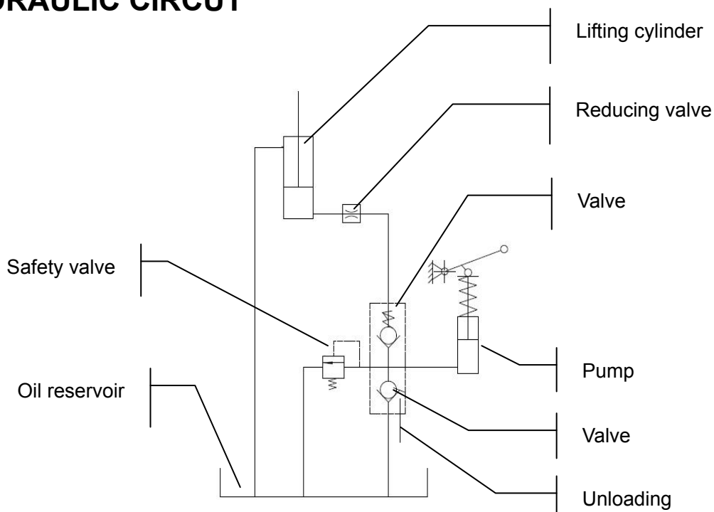
Fig. 7: Hydraulic circuit
